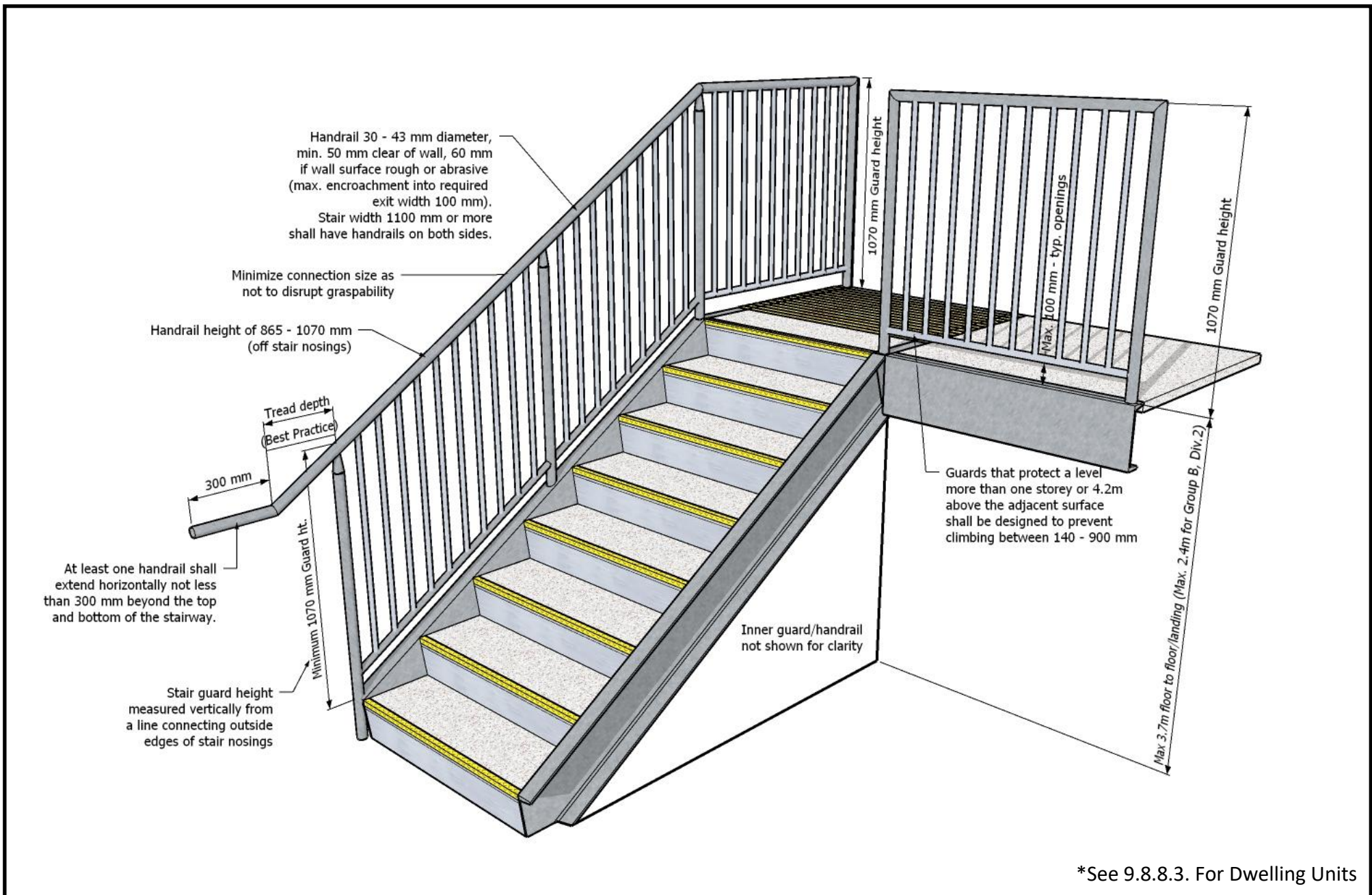
Figure 2 Handrail & Guard Integrated BC Building Code 2018
